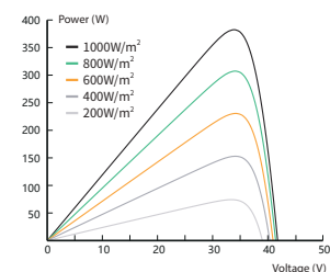
Power-Voltage Curve(380W)
